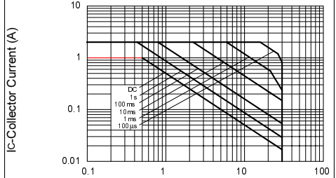
Safe Operating Area
